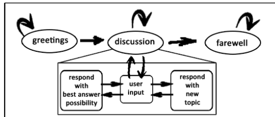
Fig. 2 Dialog System Template
